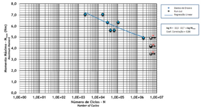
Figure 12 - Maximum moment (N.m) versus number of cycles graph obtained for the dynamic loading test of zygomatic implants.
